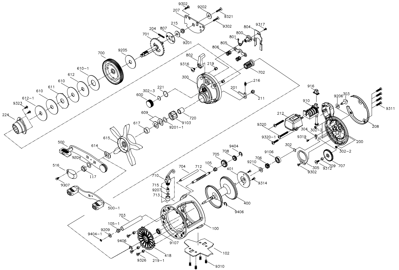
DMG - 20L (1 of 2) Spare Parts
