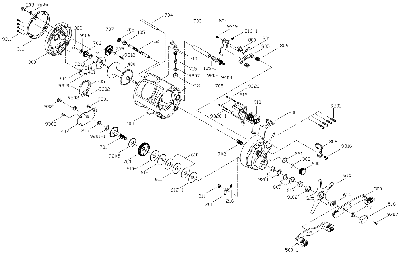
MA - 20DX Spare Parts
