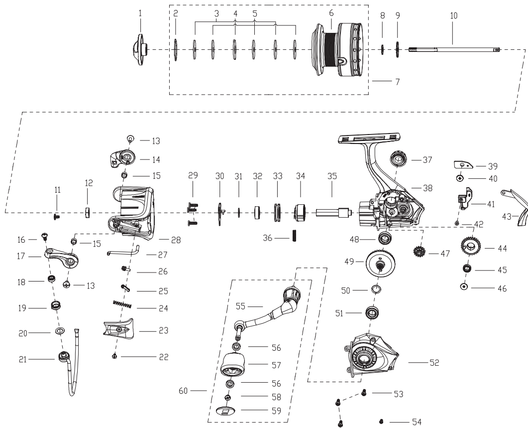
PARTS LIST OF MAXSTXSP20
