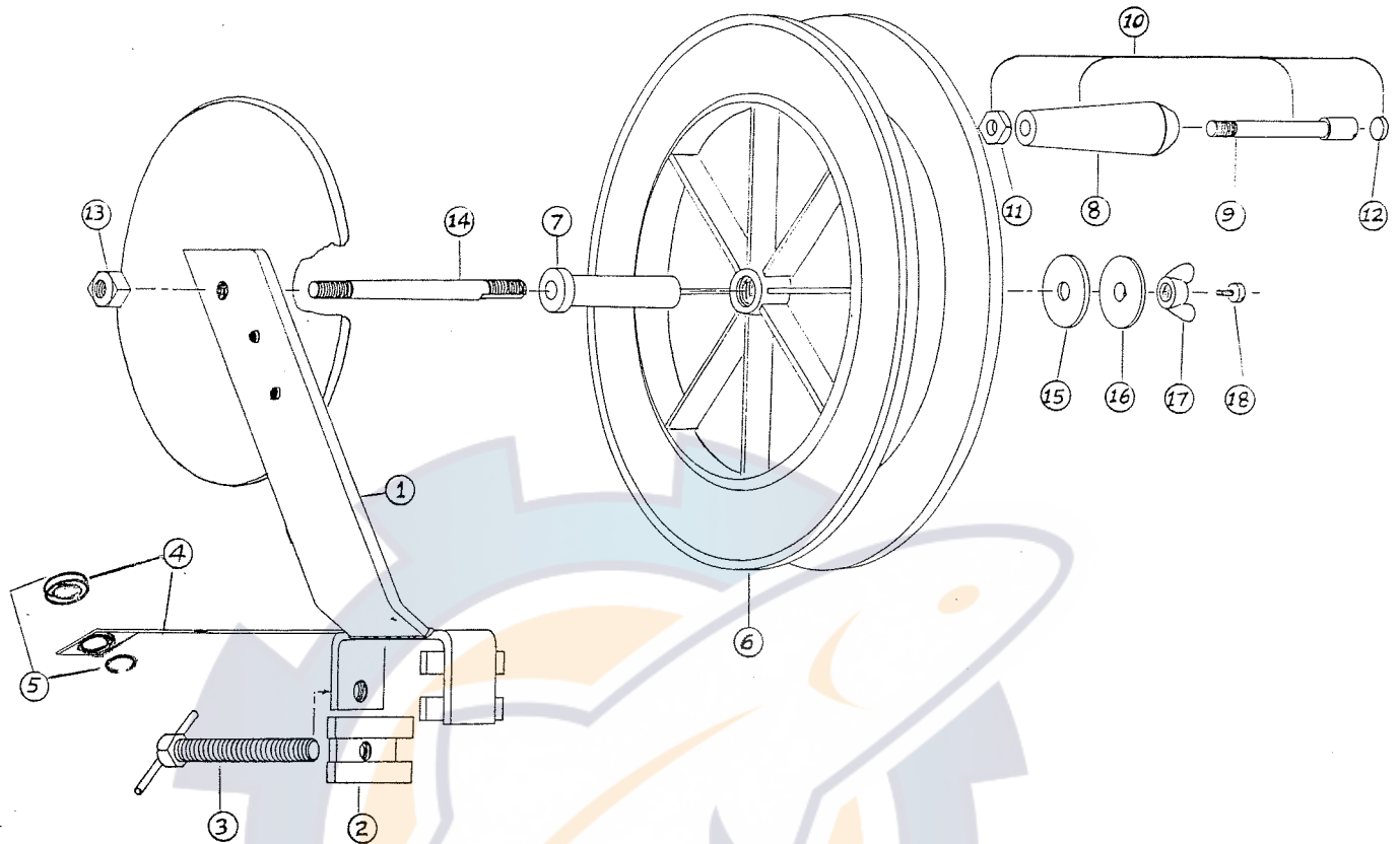
Parts for Economy Winch
