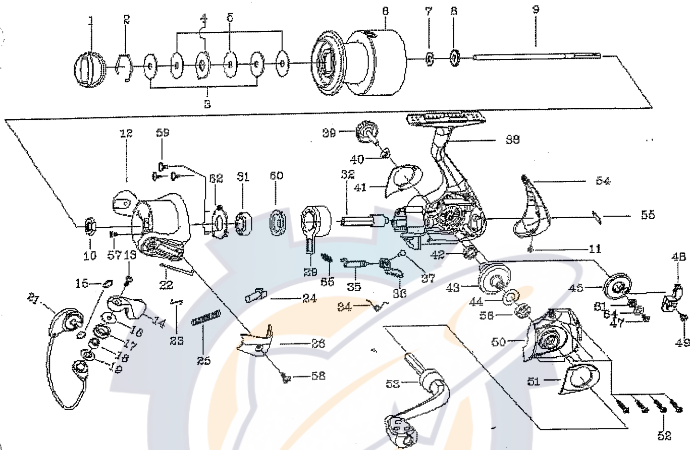
C302/303/304/305/306 FD
