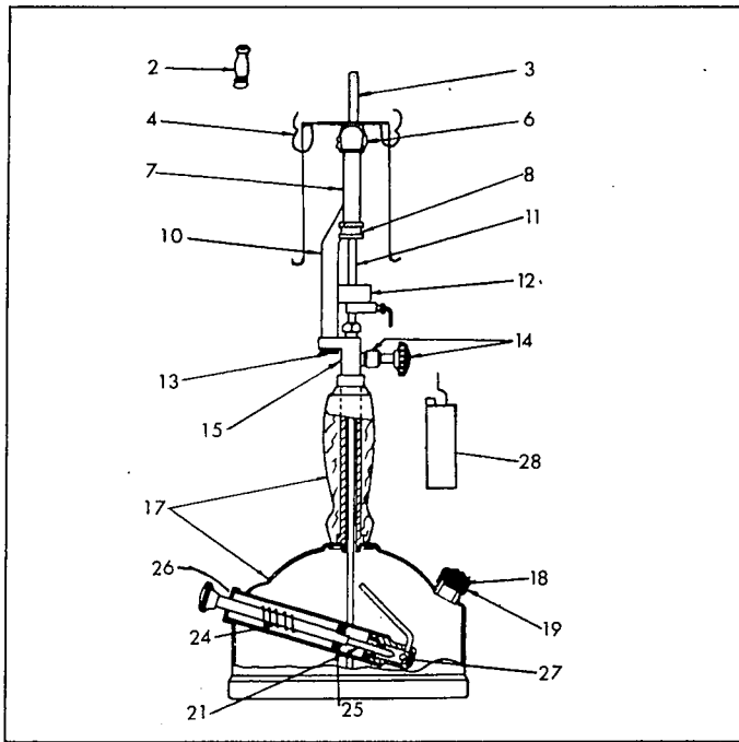
MODEL 156, 158, 159, 159X
