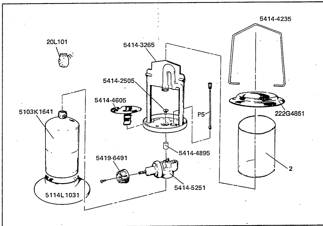
MODEL 5414 LANTERN
