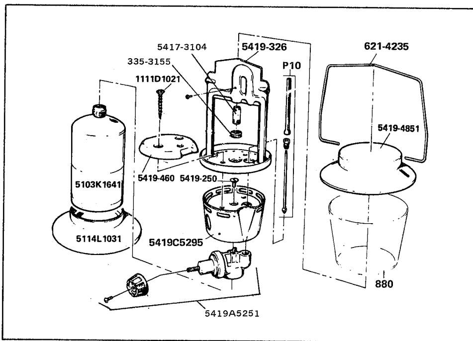
MODEL 5419A LANTERN
