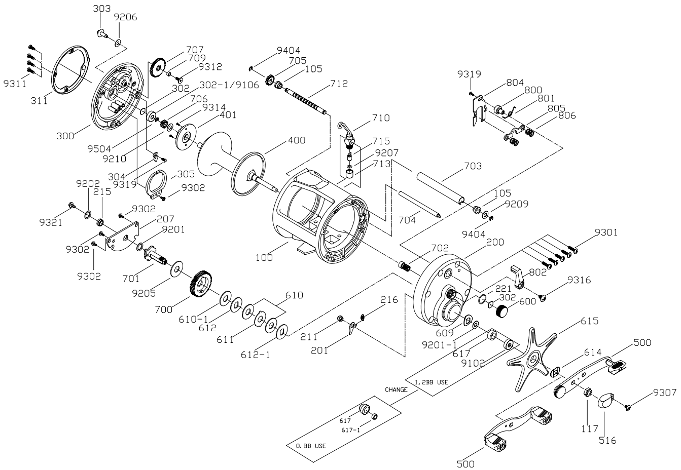
DZ - 30L Spare Parts
