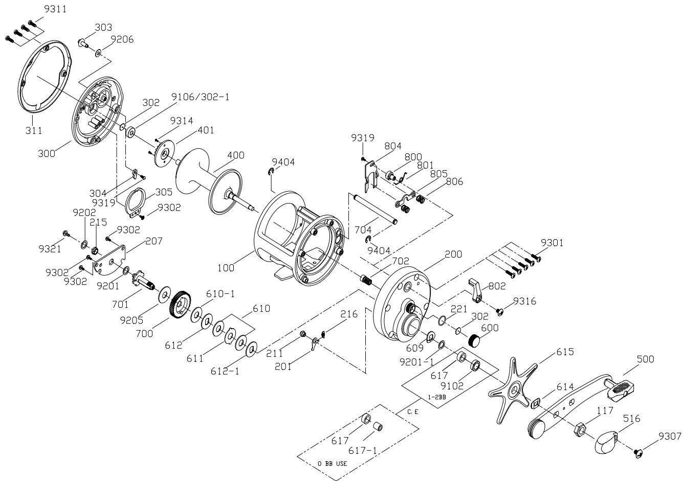
DZ - 45C Spare Parts
