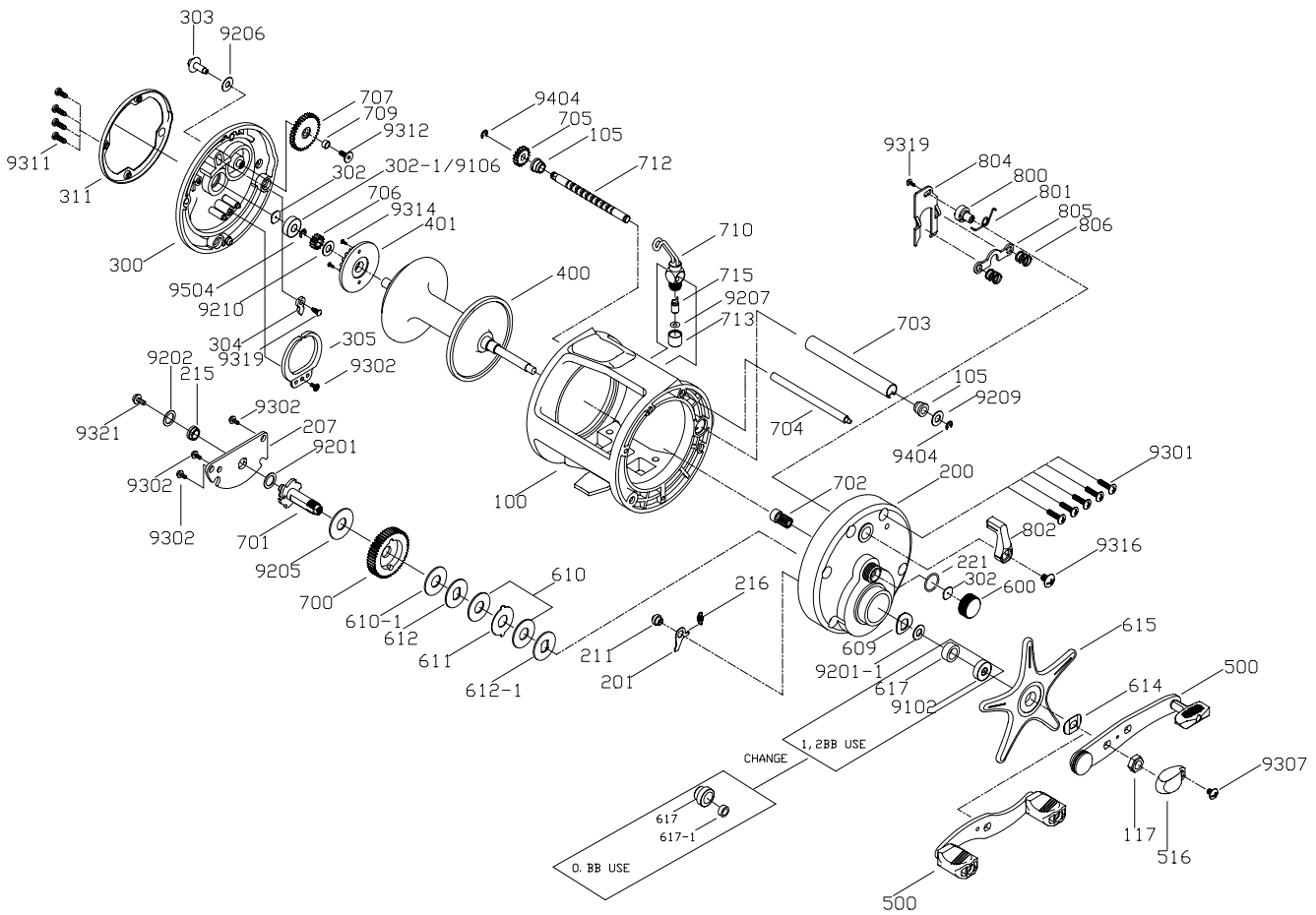
DZ - 45L Spare Parts
