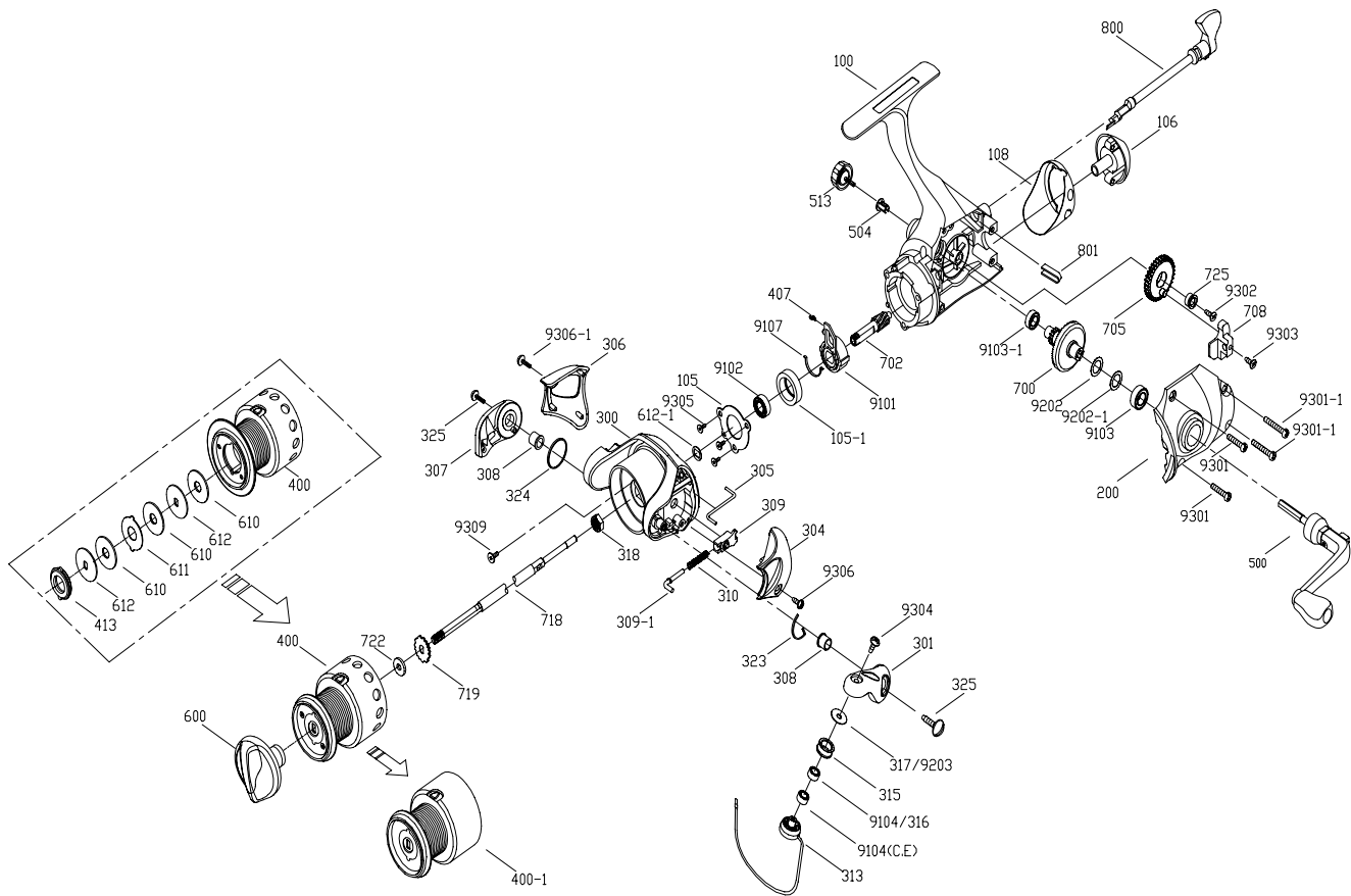
FHS - 30 Spare Parts
