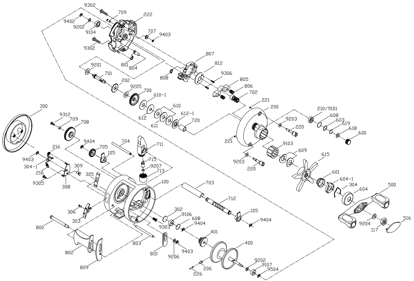
X - 400 (1 of 2) Spare Parts
