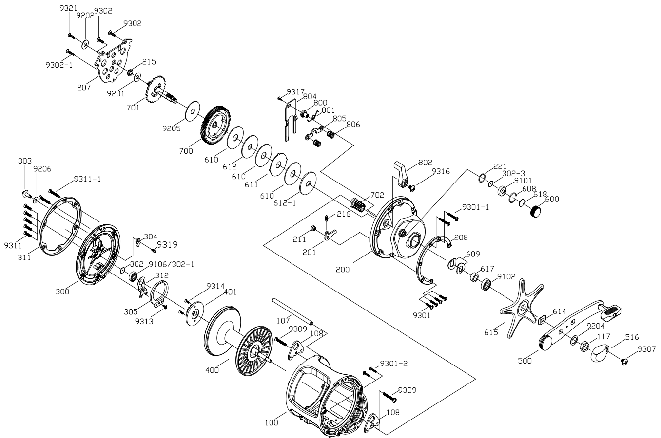
SD - 55W Spare Parts
