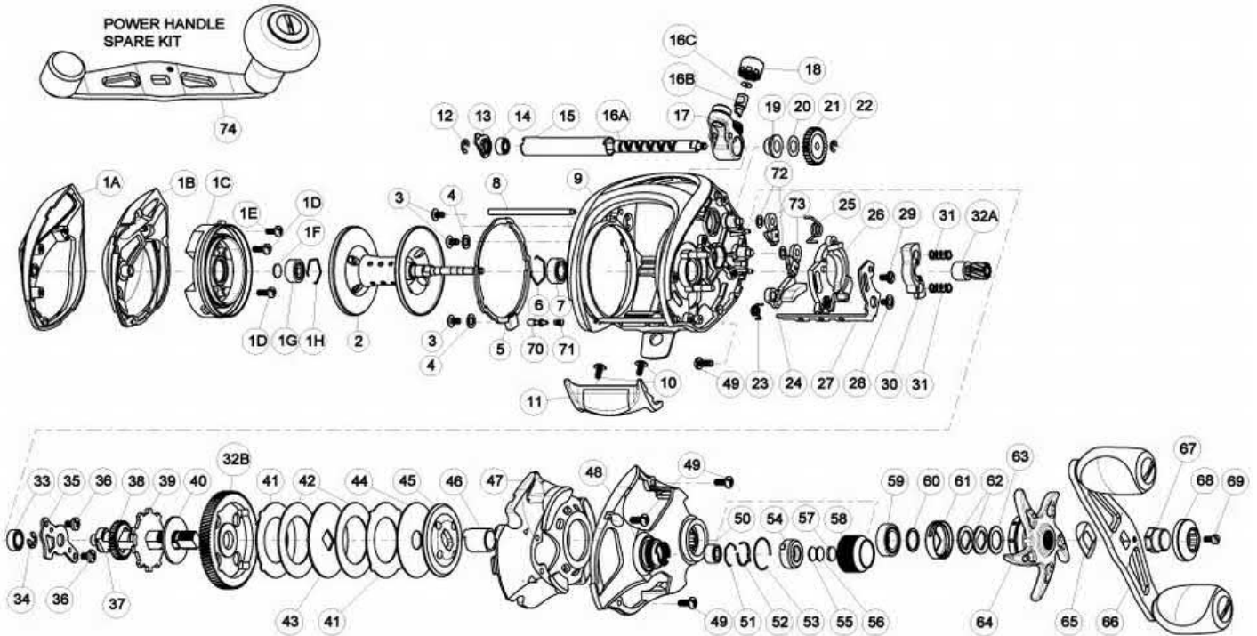
Quantum EX300PPT Bait Cast Reel Part List
