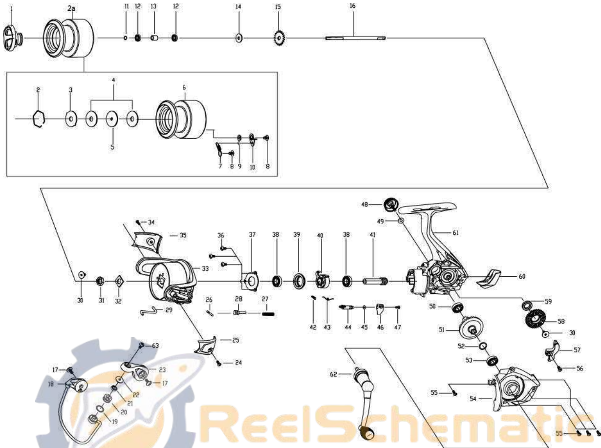
Quantum Five20 Spinning Reel Part List
