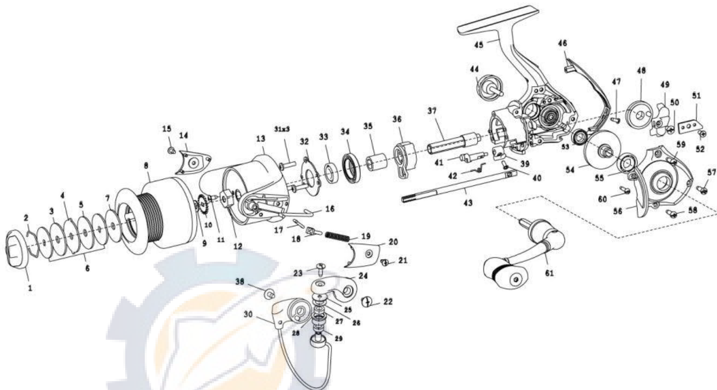
Quantum Response RE40F Spinning Reel Part List
