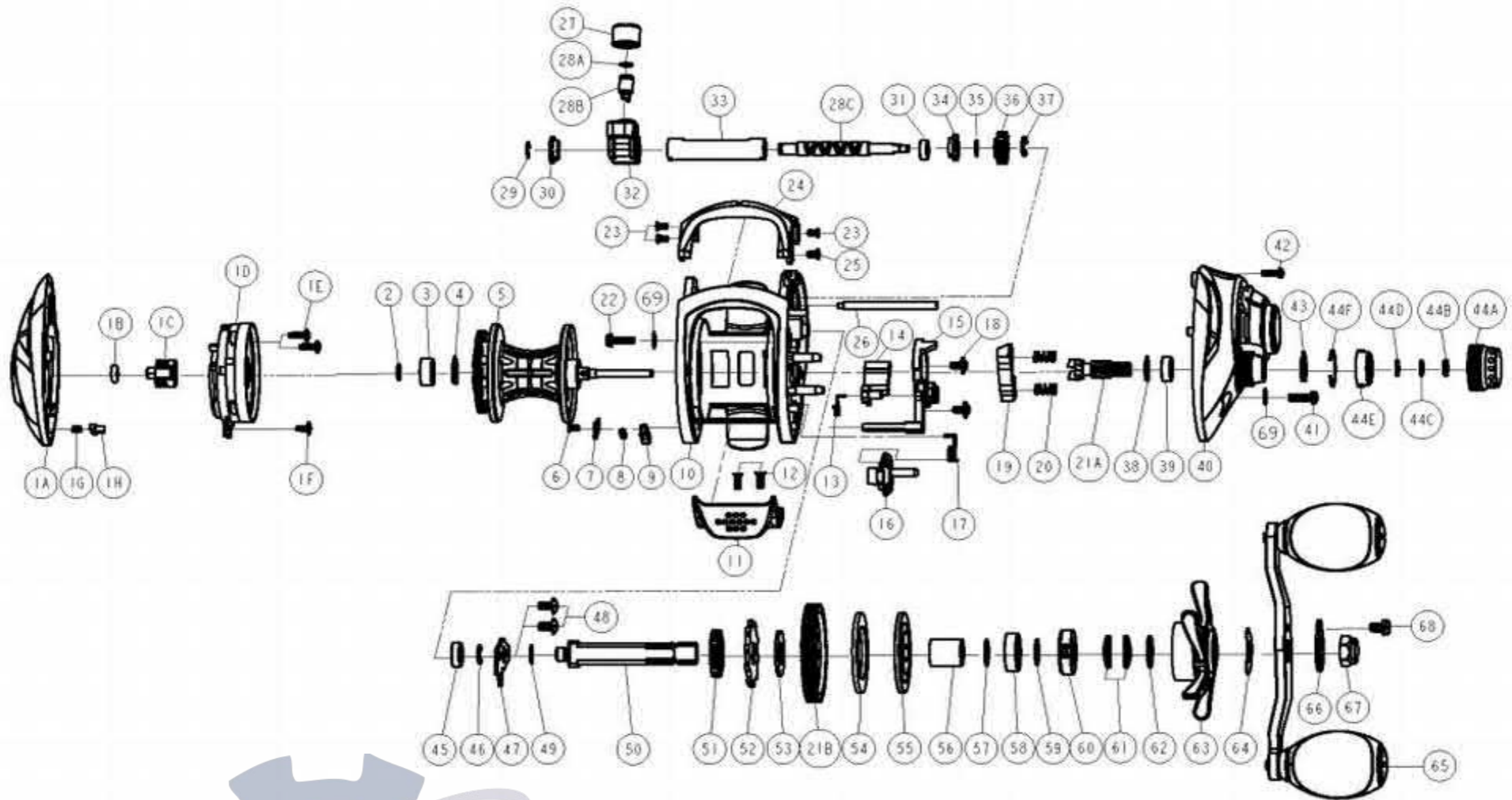
Quantum Energy T100SPTMG Baitcast Reel Part List
