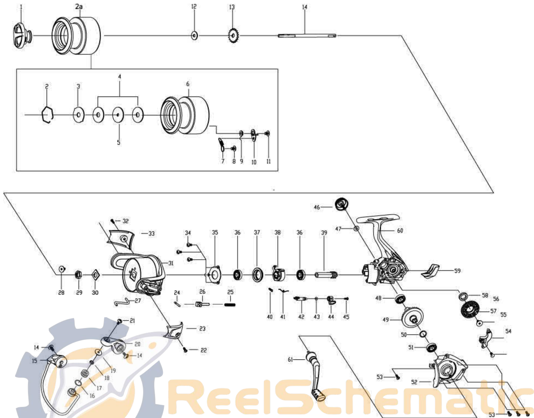
Quantum Vibe30 Spinning Reel Part List
