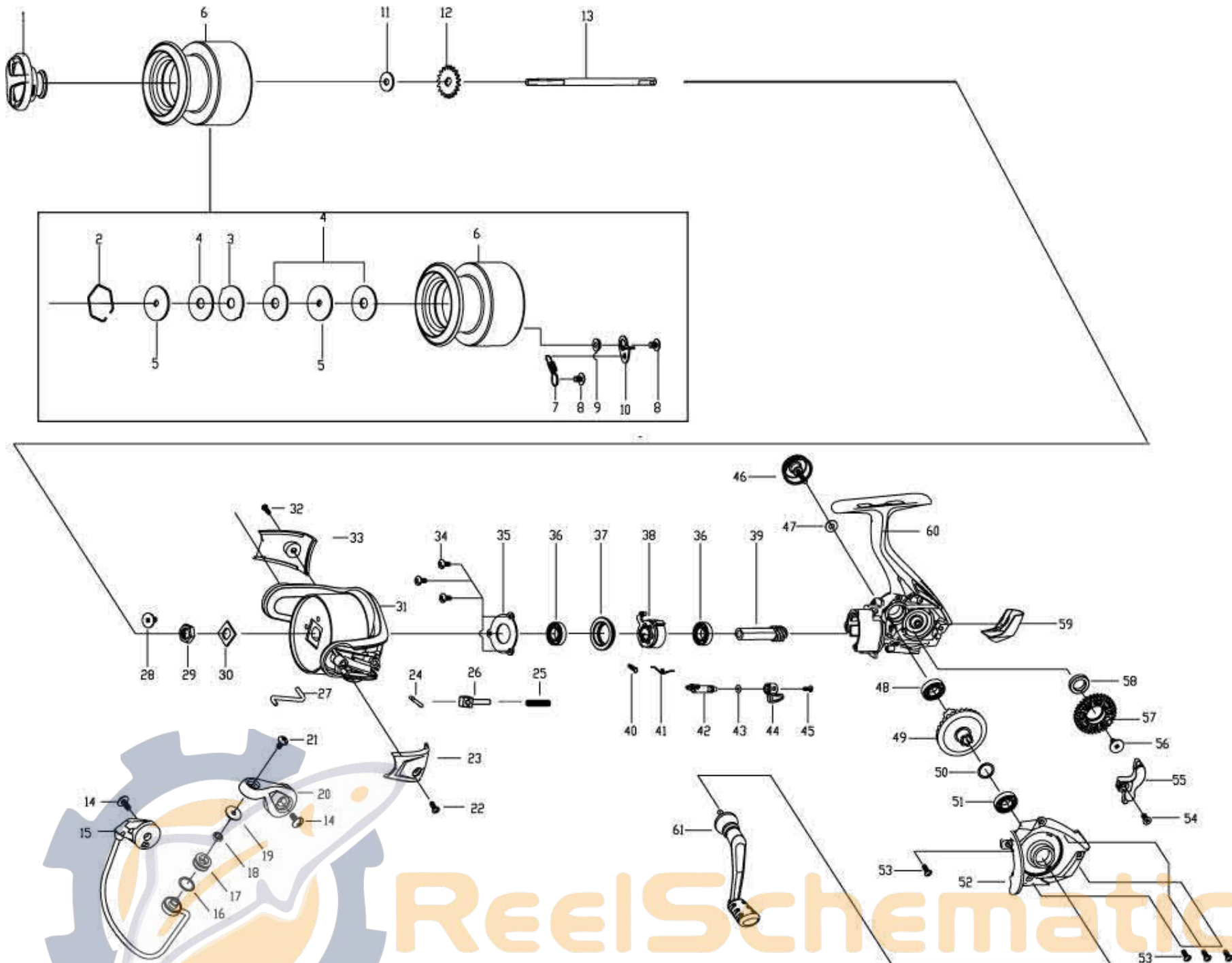
Quantum Vibe40 Spinning Reel Part List
