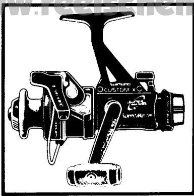
EXPLODED PARTS VIEW Speed Master CX2500SQ
